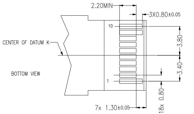
RECOMMENDED LAYOUT DETAIL MATING TRANSCEIVER PCB
