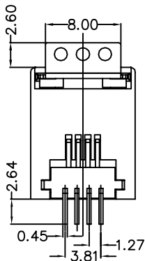
BACK VIEW
