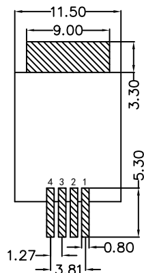
RECOMMENDED PCB LAYOUT VIEWED FROM COMPONENT SIDE
