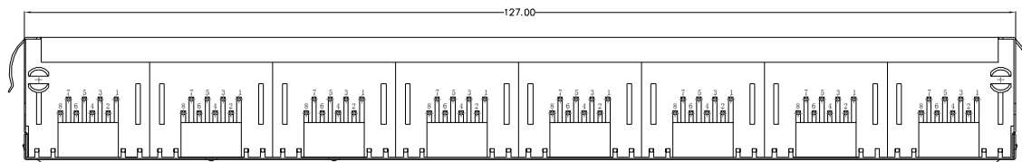
BOTTOM VIEW
