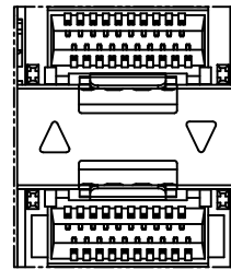
TYPE8_2 OUTER LIGHT PIPE 10732321F003 10732321F004
