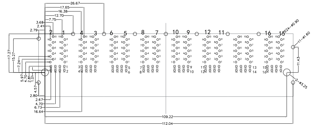
RECOMMENDED PCB LAYOUT VIEWED FROM COMPONENT SIDE
