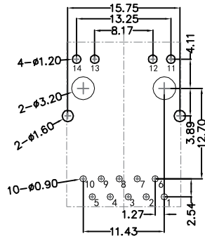
RECOMMENDED PCB LAYOUT VIEWED FROM COMPONENT SIDE
